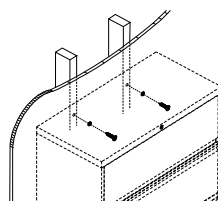
Wall anchoring
